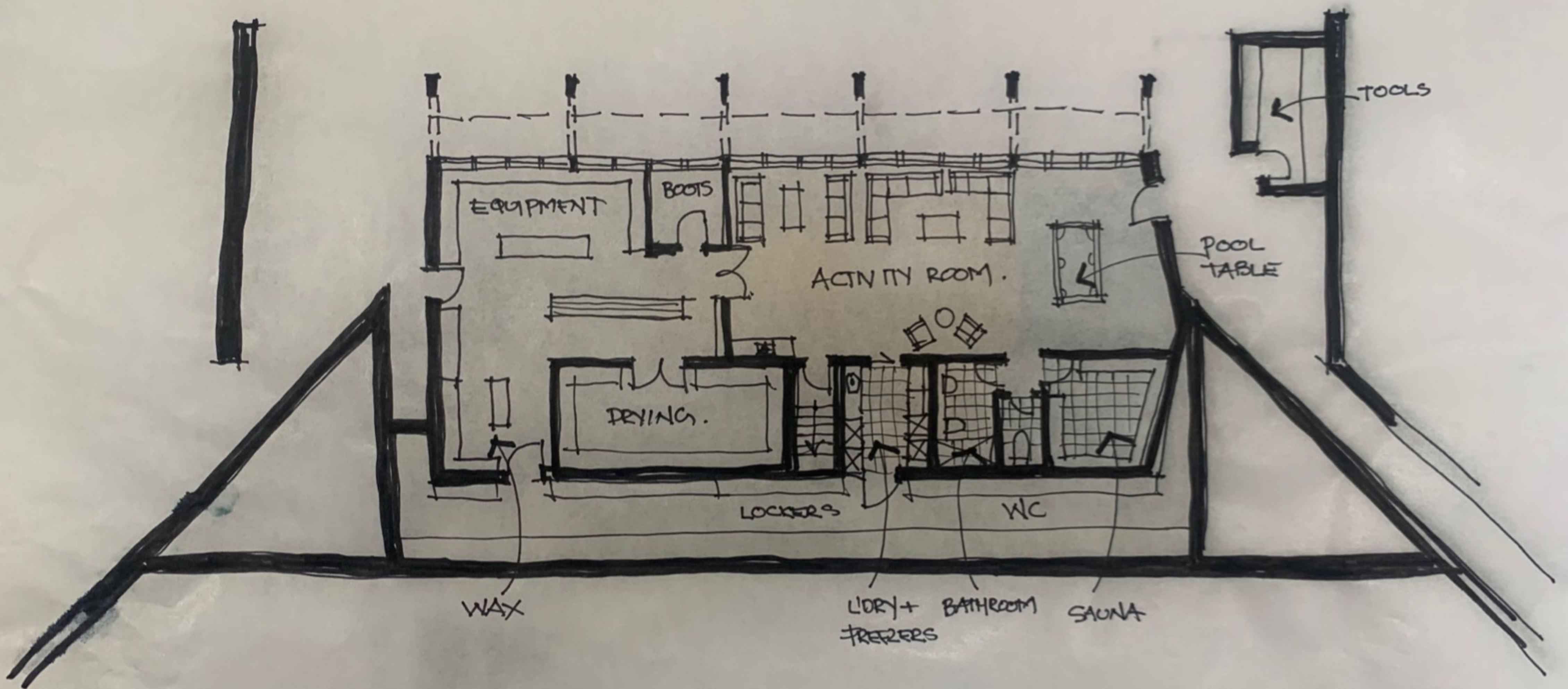
PROPOSED FLOOR PLAN 1:100
